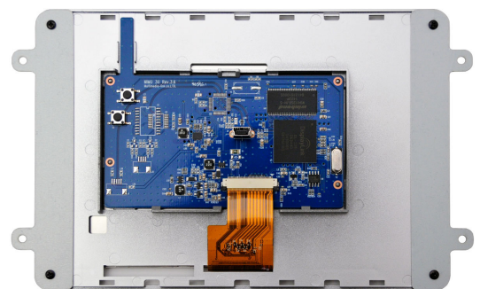
UM-760R-OF Back view
