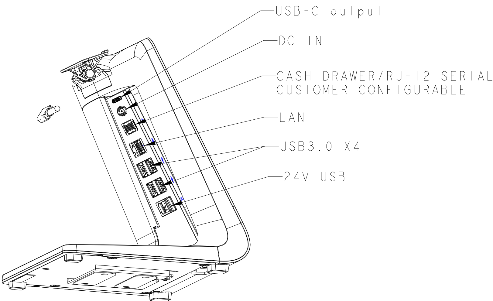
I/O DEFINITION (CABLE COVER DOOR RMOVED)
