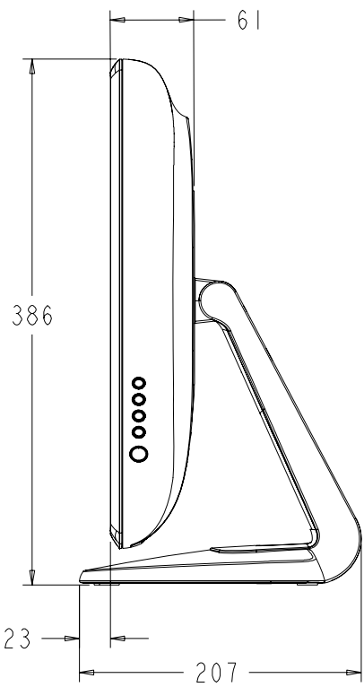
TILT -5° FROM VERTICAL
