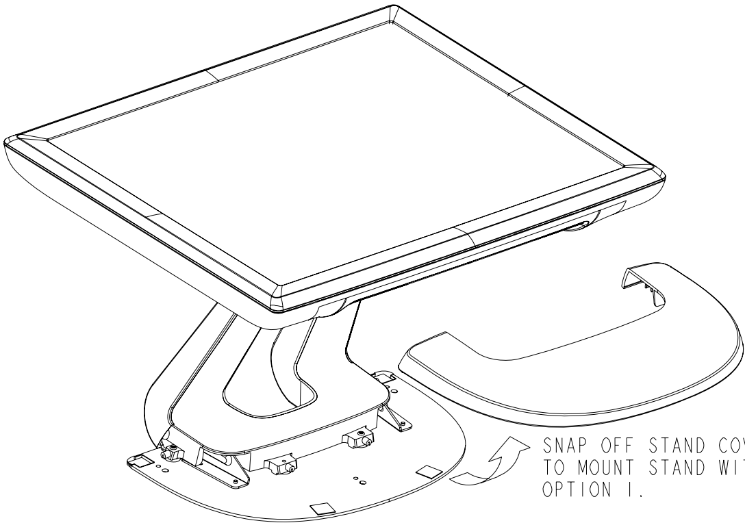
MOUNT OPTION 1
